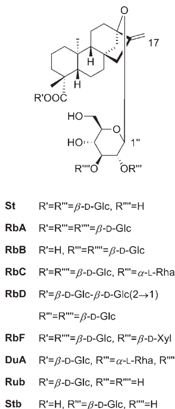
Chart 1. Structures of Stevioside, Rebaudioside A, Rebaudioside B, Rebaudioside C, Rebaudioside D, Rebaudioside F, Dulcoside A, Rubusoside, and Steviolbioside a
